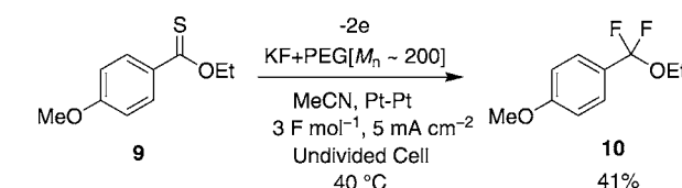
Scheme 2. Anodic difluorination of thionoester using the KF/PEG system.
