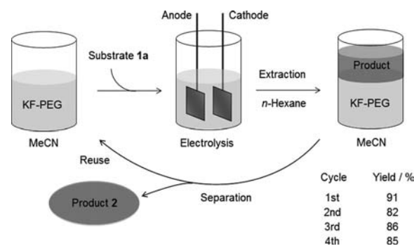
Figure 3. Experimental schematic for anodic fluorination of 1a . Data for the reusability of electrolytic solution containing KF and PEG.
