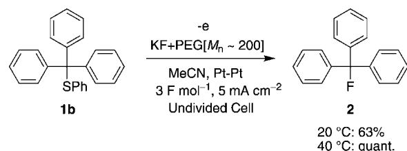
Scheme 1. Anodic fluorination of phenyltriphenylmethanesulfide using the KF/PEG system.
